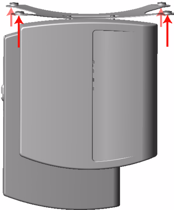
Figure 2-14 Mounting the AP-600 to the Ceiling
