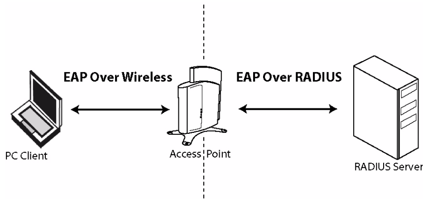
Figure 4-17 RADIUS Authentication Illustrated
